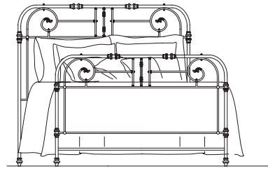
GARDEN GATE BED 192310 / 5/0 Queen 63w x 85d x 59h 192320 / 6/6 King 79w x 85d x 59h (Footboard height is 40") Height from floor to bottom of box spring is 6". Shown on page: 14
